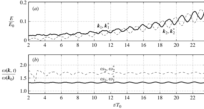
FIGURE 6. (a) Normalized energy evolution of the dominant modes \mathbf{k}_1 = (1, \frac{4}{3}) , \mathbf{k}_1^* = (1, -\frac{4}{3}) , \mathbf{k}_2 = (2, \frac{4}{3}) and \mathbf{k}_2^* = (2, -\frac{4}{3}) . (b) Evolution of the frequency \omega . The initial perturbation corresponds to (p, q) = (0, \frac{4}{3}) , (ak)_0 = 0.2985 and \epsilon = 0.05 .
