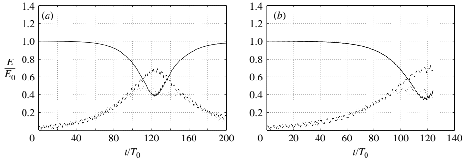
FIGURE 2. Normalized energy evolution of the fundamental mode and satellites: (k, 0) (solid line), (0.8k, 0) (dashed line) and (1.2k, 0) (dotted line). (a) An initial steepness (ak)_0 = 0.11 showing the periodic modulations. (b) An initial steepness (ak)_0 = 0.1125 showing the numerical blow-up of the simulation corresponding to breaking.
