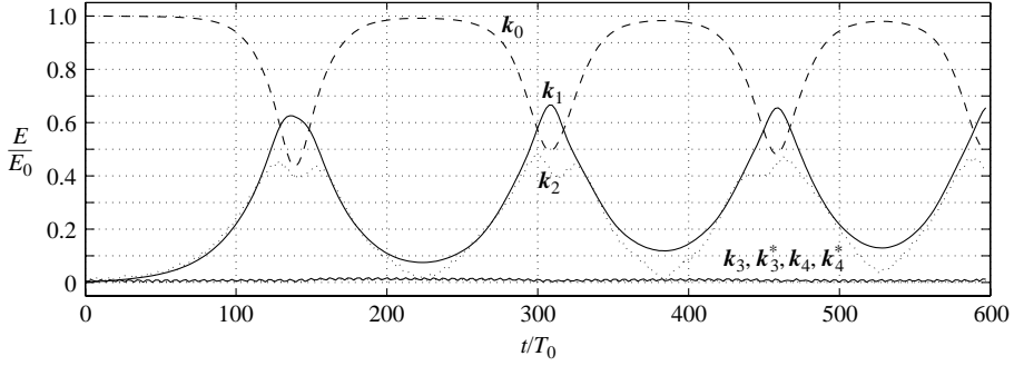
FIGURE 16. Normalized energy evolution of the main modes: \mathbf{k}_0 = (1, 0) , \mathbf{k}_1 = (\frac{3}{4}, 0) , \mathbf{k}_2 = (\frac{5}{4}, 0) , \mathbf{k}_3 = (\frac{3}{4}, 1.612) , \mathbf{k}_4 = (\frac{7}{4}, 1.612) , \mathbf{k}_3^* = (\frac{7}{4}, -1.612) , \mathbf{k}_4^* = (\frac{3}{4}, -1.612) and \mathbf{k}_4 = (\frac{7}{4}, 1.612) . The initial wave field is a Stokes wave with (ak)_0 = 0.13 and the initial perturbations are \mathbf{k}_1 , \mathbf{k}_2 , \mathbf{k}_3 and \mathbf{k}_3^* . \epsilon = 0.01 .
