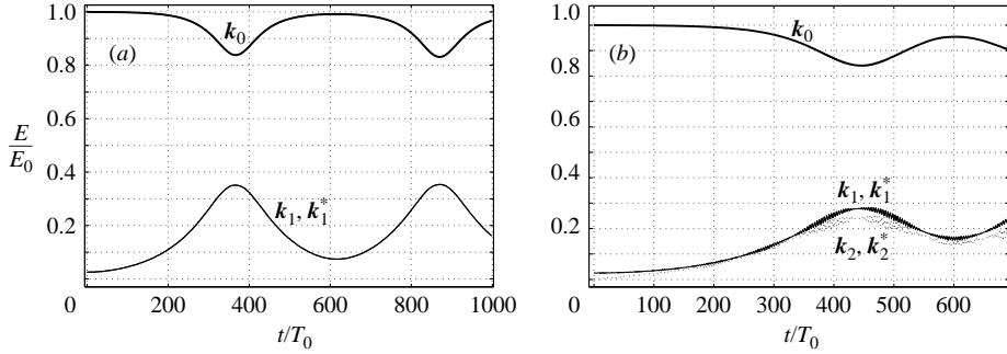
FIGURE 8. Normalized energy evolution of the fundamental mode and satellites. (a) \mathbf{k}_0 = (1, 0) , \mathbf{k}_1 = (\frac{3}{2}, q) and \mathbf{k}_1^* = (\frac{3}{2}, -q) with (ak)_0 = 0.13 , q = 1.621 , \epsilon = 0.05 . (b) \mathbf{k}_0 = (1, 0) , \mathbf{k}_1 = (1, q) , \mathbf{k}_1^* = (1, -q) , \mathbf{k}_2 = (2, q) and \mathbf{k}_2^* = (2, -q) with (ak)_0 = 0.13 , q = 1.5975 , \epsilon = 0.05 .
