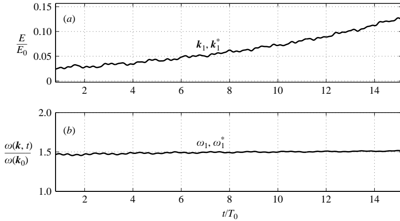
FIGURE 3. (a) Normalized energy evolution of the dominant modes \mathbf{k}_1 = (\frac{3}{2}, \frac{4}{3}) and \mathbf{k}_1^* = (\frac{3}{2}, -\frac{4}{3}) . (b) Evolution of the frequency \omega . The initial perturbation corresponds to (p, q) = (\frac{1}{2}, \frac{4}{3}) , (\bar{a}k)_0 = 0.2985 and \epsilon = 0.05 .
