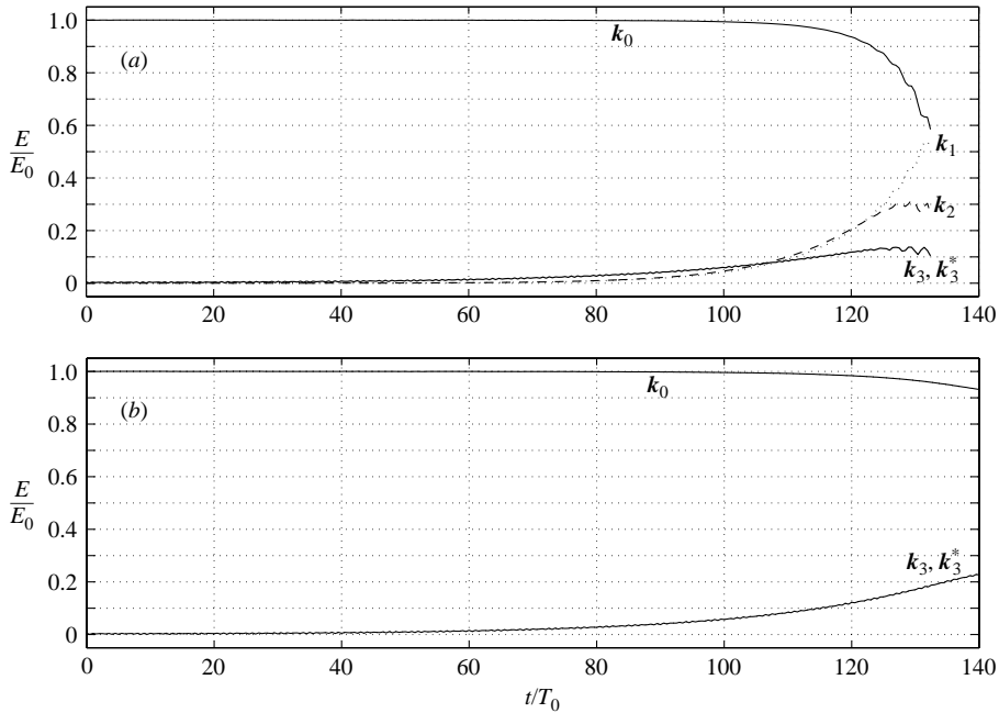
FIGURE 17. Normalized energy evolution of the main modes: \mathbf{k}_0 , \mathbf{k}_1 = (\frac{3}{4}, 0) , \mathbf{k}_2 = (\frac{5}{4}, 0) , \mathbf{k}_3 = (\frac{3}{2}, 1.53) and \mathbf{k}_3^* = (\frac{3}{2}, -1.53) . The initial wave field is a Stokes wave with (ak)_0 = 0.20 and the initial perturbations are (a) \mathbf{k}_1 , \mathbf{k}_2 (with \epsilon = 0.0001 ), \mathbf{k}_3 and \mathbf{k}_3^* (with \epsilon = 0.01 ), (b) \mathbf{k}_3 and \mathbf{k}_3^* only.
