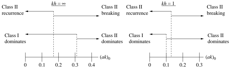
FIGURE 21. Steepness threshold for recurrence vs. breaking and predominance of class I instabilities vs. class II instabilities for kh = \infty and kh = 1 .
