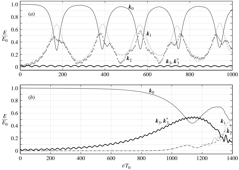
FIGURE 13. Normalized energy evolution of the main modes: \mathbf{k}_0 = (1, 0) , \mathbf{k}_1 = (\frac{5}{6}, 0) , \mathbf{k}_2 = (\frac{7}{6}, 0) , \mathbf{k}_3 = (\frac{3}{2}, 1.645) , \mathbf{k}_3^* = (\frac{3}{2}, -1.645) . The initial wave field is a Stokes wave with (ak)_0 = 0.10 and the initial perturbations are: (a) \mathbf{k}_1 , \mathbf{k}_2 , \mathbf{k}_3 and \mathbf{k}_3^* and (b) \mathbf{k}_3 and \mathbf{k}_3^* only. \epsilon = 0.025 .
