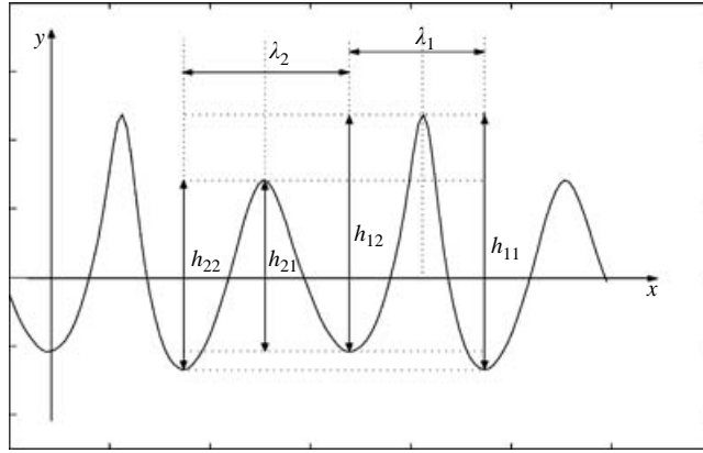
FIGURE 4. Definition of Su's geometric parameters.
