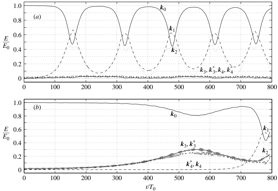
FIGURE 15. Normalized energy evolution of the main modes: \mathbf{k}_0 = (1, 0) , \mathbf{k}_1 = (\frac{3}{4}, 0) , \mathbf{k}_2 = (\frac{5}{4}, 0) , \mathbf{k}_3 = (1, 1.5975) , \mathbf{k}_4 = (2, 1.5975) , \mathbf{k}_3^* = (1, -1.5975) , \mathbf{k}_4^* = (2, -1.5975) . The initial wave field is a Stokes wave with (ak)_0 = 0.13 and the initial perturbations are: (a) \mathbf{k}_1 , \mathbf{k}_2 , \mathbf{k}_3 and \mathbf{k}_3^* , (b) \mathbf{k}_3 and \mathbf{k}_3^* only. \epsilon = 0.025 .
