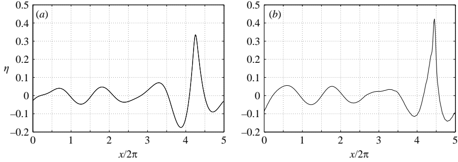
FIGURE 1. Free-surface profiles of an evolved wave group with five waves in the modulation. To the initial Stokes wave has been added two small sidebands at t/T_0 = 0 . (a) An evolved wave group with initial steepness (ak)_0 = 0.11 at t/T_0 = 123 , in this case the evolution is periodic. (b) An initial steepness (ak)_0 = 0.1125 at t/T_0 = 123 , this case leads to breaking.
