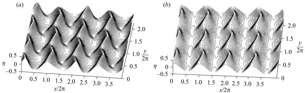
FIGURE 5. Free surface elevation corresponding to (a) figure 3 at t/T_0 = 18 and (b) figure 5 at t/T_0 = 23 .
