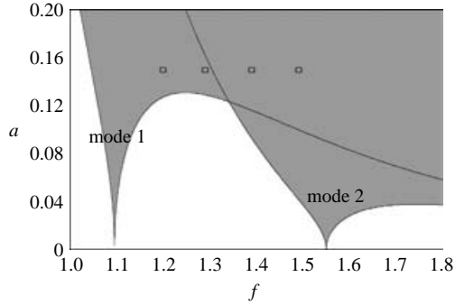
FIGURE 24. Margin of stability of the two first cross-wave modes. The solid lines are neutral wavenumber amplitude as a function of wavenumber frequency while the grey areas represent unstable regions and correspond to a growth of the cross-waves. The wavenumber parameters correspond to the experimental setup by Collard & Caulliez while the squares indicate the location of some of their experiments.
