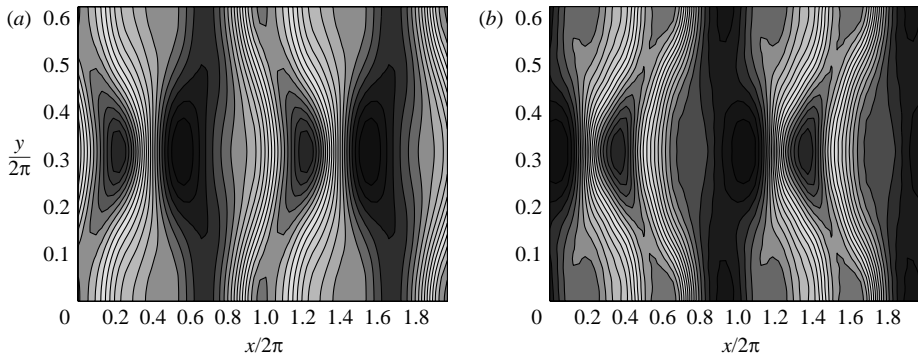
FIGURE 11. Oscillating horseshoe patterns corresponding to figure 8(b) at (a) 360T_0 and (b) 504T_0 .
