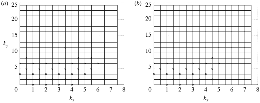
FIGURE 10. Wave-vector spectra of the wave fields corresponding to (a) figure 9(a), (b) figure 9(d). The components whose energy is larger than 10^{-6} are depicted as a circle.
