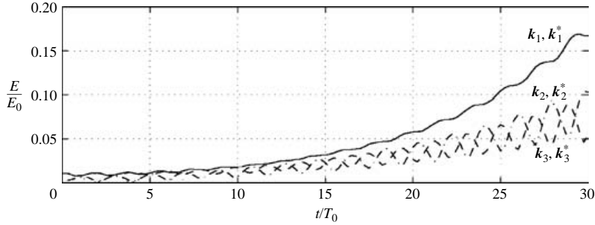
FIGURE 20. Coexistence of two class II instabilities for kh=1 and (ak)_0=0.20 . The dominant modes of the instabilities corresponding to phase-locked horseshoe patterns are \mathbf{k}_1 = (\frac{3}{2}, 0.91) , \mathbf{k}_1^* = (\frac{3}{2}, -0.91) and those corresponding to oscillating patterns are \mathbf{k}_2 = (1.0, 0.91) , \mathbf{k}_2^* = (1.0, -0.91) and \mathbf{k}_3 = (2, 0.91) , \mathbf{k}_3^* = (2, -0.91) . The instabilities are triggered with \epsilon = 0.02 .
