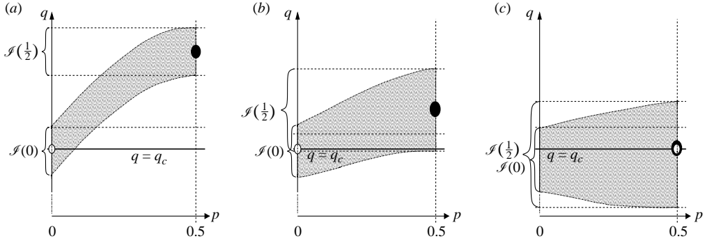
FIGURE 23. Schematic instability diagrams of class II focusing on the unstable region with 0 \leq p \leq 0.5 . The different cases depict the three regimes in infinite depth corresponding typically to (a) (ak)_0 < 0.17 , (b) 0.17 < (ak)_0 < 0.2 and (c) (ak)_0 > 0.2 . The black dot labels the most unstable perturbation of class II and the white dot labels the most unstable mode along the line q = q_c .
