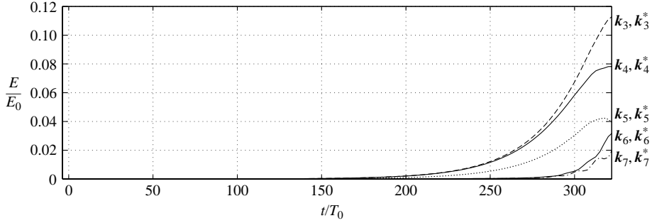
FIGURE 12. Normalized energy evolution of the dominant modes of the instabilities: \mathbf{k}_3 = (\frac{3}{5}, 1.53) , \mathbf{k}_3^* = (\frac{3}{5}, -1.53) , \mathbf{k}_4 = (\frac{5}{4}, 1.53) , \mathbf{k}_5^* = (\frac{7}{4}, -1.53) , \mathbf{k}_4^* = (\frac{5}{4}, -1.53) , \mathbf{k}_5 = (\frac{7}{4}, 1.53) , \mathbf{k}_6 = (1, 1.53) , \mathbf{k}_7^* = (2, -1.53) , \mathbf{k}_7 = (2, 1.53) , \mathbf{k}_6^* = (2, -1.53) . The initial wave field is a Stokes wave with (ak)_0 = 0.20 plus the whole discrete spectrum of class II instabilities corresponding to p = 0, \frac{1}{4}, \frac{1}{2}, \frac{3}{4} . \epsilon = 0.0001 .
