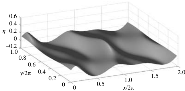
FIGURE 19. Surface elevation corresponding to figure 18 at t/T_0 = 160 .
