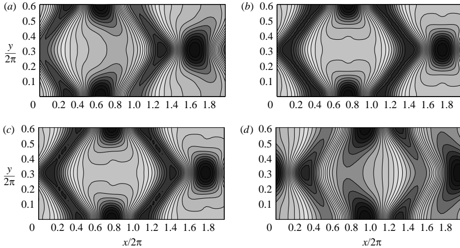
FIGURE 9. Iso-elevation plots corresponding to figure 8(a) at time (a) t/T_0 = 340 , (b) t/T_0 = 368 , (c) t/T_0 = 372 and (d) t/T_0 = 420 .
