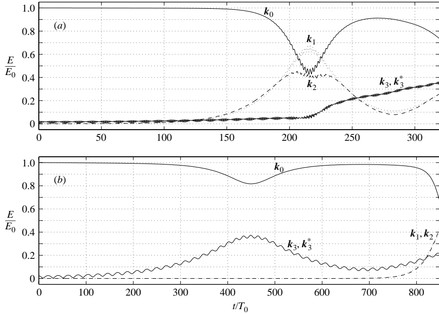
FIGURE 14. Normalized energy evolution of the main modes: \mathbf{k}_0 = (1, 0) , \mathbf{k}_1 = (\frac{3}{4}, 0) , \mathbf{k}_2 = (\frac{5}{4}, 0) , \mathbf{k}_3 = (\frac{3}{2}, 1.621) , \mathbf{k}_3^* = (\frac{3}{2}, -1.621) . The initial wave field is a Stokes wave with (ak)_0 = 0.13 and the initial perturbations are: (a) \mathbf{k}_1 , \mathbf{k}_2 , \mathbf{k}_3 and \mathbf{k}_3^* and (b) \mathbf{k}_3 and \mathbf{k}_3^* only. \epsilon = 0.025 .
