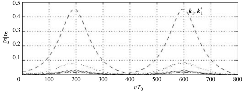
FIGURE 18. Recurrence for class II instability with (p, q) = (\frac{1}{2}, 0.98) , kh = 1 , (ak)_0 = 0.11 . The instability with dominant modes \mathbf{k}_1 = (\frac{3}{2}, 0.98) and \mathbf{k}_1^* = (\frac{3}{2}, -0.98) is triggered with \epsilon = 0.05 . The other curves represent the higher-order harmonics of the instability.
