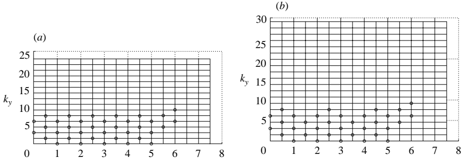
FIGURE 7. Excited modes for two different transverse grid resolutions in a simulation with (ak)_0 = 0.2 and dominant modes \mathbf{k}_1 = (\frac{3}{2}, 1.53) and \mathbf{k}_1^* = (\frac{3}{2}, -1.53) . These spectra correspond to the end of the phase of increase of the satellites when the surface elevation shows fully developed horseshoe patterns. (a) 16 modes in the transverse direction are solved with 64 collocation points and (b) 20 modes in the transverse direction are solved with 80 collocation points.
