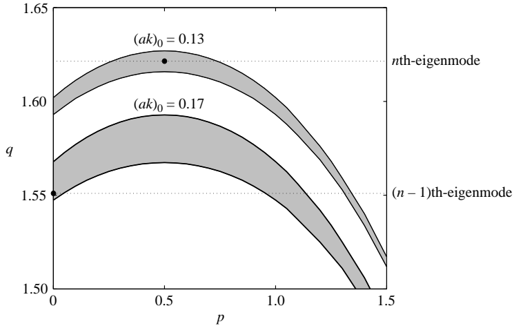
FIGURE 26. Class II instability diagrams for wave steepness (ak)_0 = 0.13 and (ak)_0 = 0.17 . The horizontal lines correspond to two consecutive eigenmodes of the numerical channel considered while the dots represent the most unstable perturbation along those horizontal lines.
