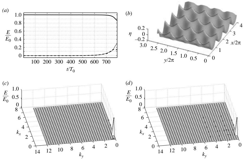
FIGURE 25. Evolution of a perturbed Stokes wave train of initial steepness (ak)_0 = 0.17 and \epsilon = 0.10 (the wave-vector spectrum of the initial condition is given in (c)). (a) Normalized energy evolution of the main modes \mathbf{k}_0 = (1, 0) (thick solid line), (1, \pm q_c) (thin solid line) and (2, \mp q_c) (dashed line) with q_c = 1.58 . (b) Free-surface elevation at t/T_0 = 740 . (c, d) wave-vector spectra of the free surface at t/T_0 = 0 and t/T_0 = 740 . Harmonics with energy larger than 10^{-6}E_0 are depicted as a circle.
