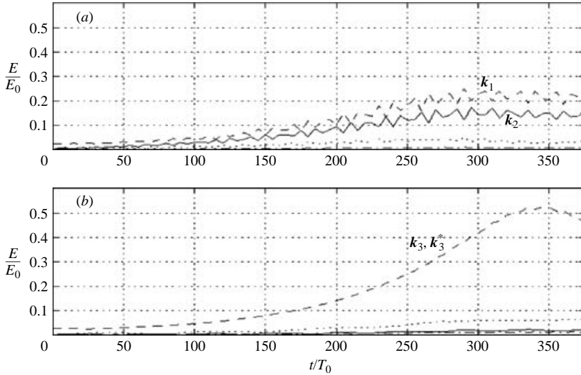
FIGURE 22. Coexistence of class I and class II instabilities for kh=1 and (ak)_0=0.10 . (a) development of the dominant modes \mathbf{k}_1 = (\frac{3}{2}, 0.31) and \mathbf{k}_2 = (\frac{1}{2}, 0.31) of the unstable class I perturbation for (p, q) = (\frac{1}{2}, 0.31) . (b) Development of the dominant modes \mathbf{k}_3 = (\frac{3}{2}, 0.992) and \mathbf{k}_3^* = (\frac{3}{2}, -0.992) of the unstable class II perturbation for (p, q) = (\frac{1}{2}, 0.992) . The instabilities are triggered with \epsilon = 0.05 .
